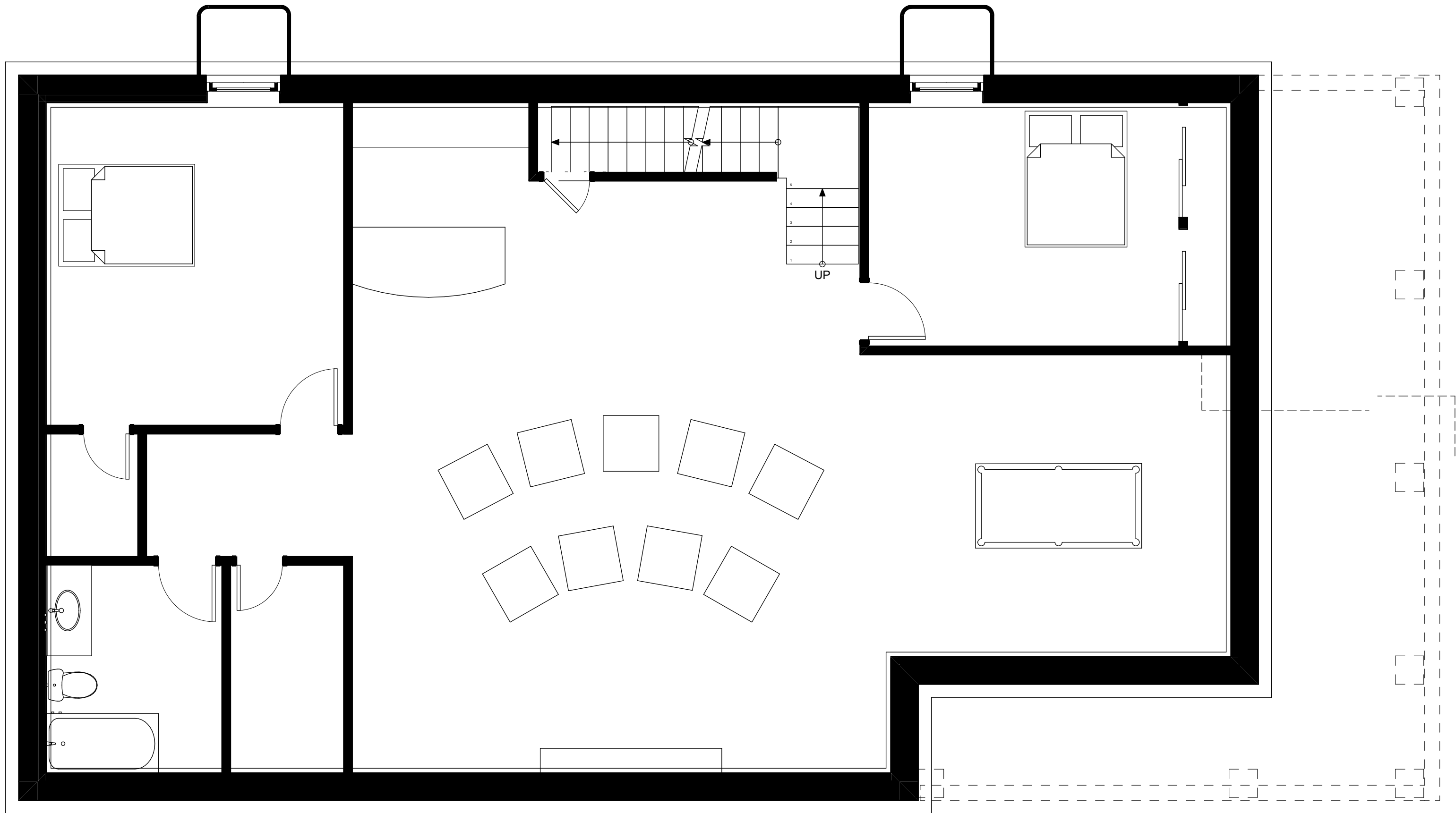
BASEMENT PLAN
